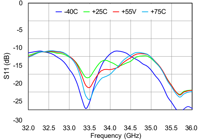
S11 vs. Frequency vs. Temperature
