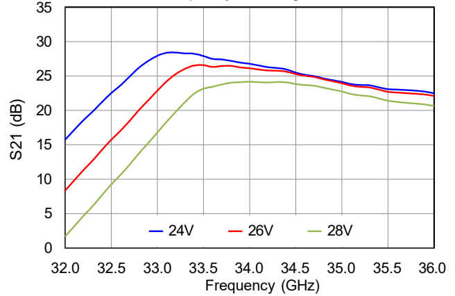
S21 vs. Frequency vs. Voltage
