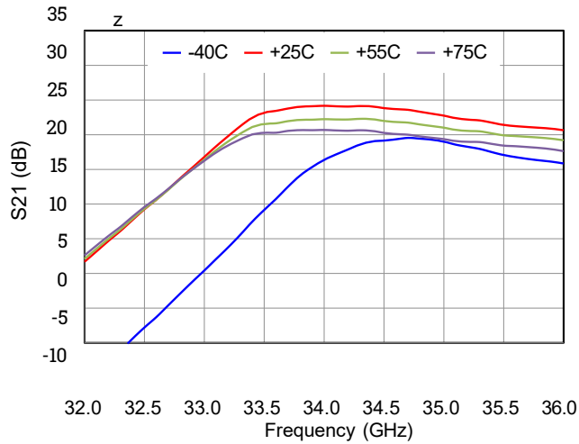
S21 vs. Frequency vs. Temperature
